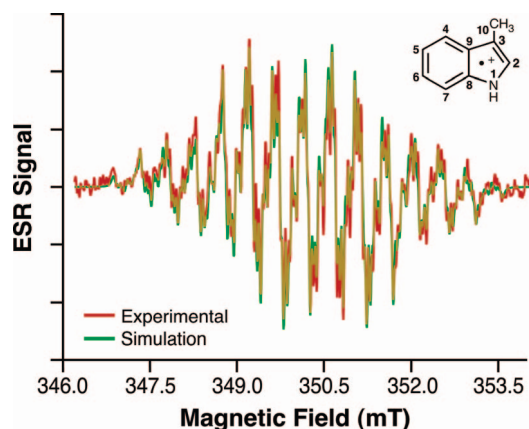
Figure 3. 3-methylindole radical cation ESR spectrum. ESR fast-flow spectrum of 3-methylindole radical cation produced in a system of 3-methylindole, \text{Ce}^{4+} , acetic acid, and \text{H}_2\text{SO}_4 having concentrations of 0.5 mM, 0.25 mM, 1.75 M, and 0.113 M, respectively. Equal volumes of aqueous solutions of 3-methylindole/acetic acid and \text{Ce}^{4+}/\text{H}_2\text{SO}_4 were mixed milliseconds before entering the ESR flat cell at a total flow rate of 50 mL/min. ESR spectra were recorded at 20 mW microwave power, 0.10 mT field modulation, 8.00 mT field sweep width, 163 ms time constant, 81 ms conversion time, and 79 scans of 1024 data points (red). Also shown is the 3-methylindole radical cation simulation spectrum with coupling constants given in Table 1 (green).
